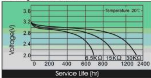
Discharge Characteristics
