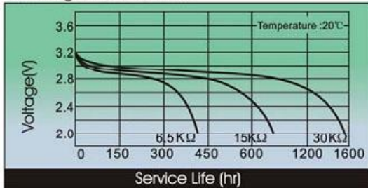
Discharge Characteristics
