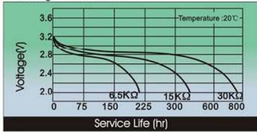
Discharge Characteristics
