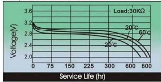
Temperature Characteristics
