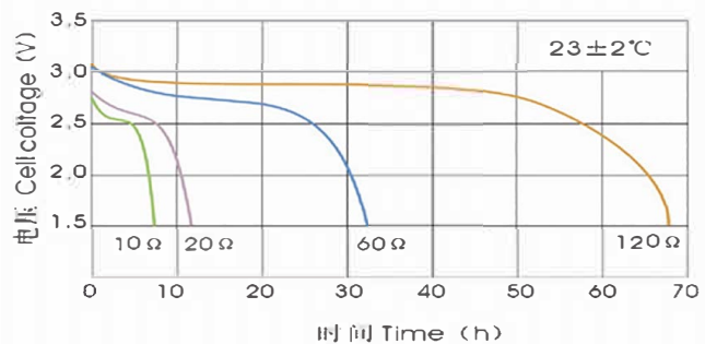
Discharge Characteristics
