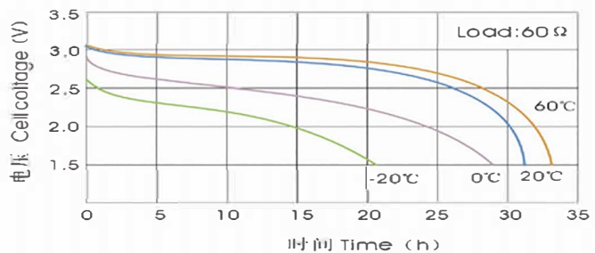
Temperature Characteristics
