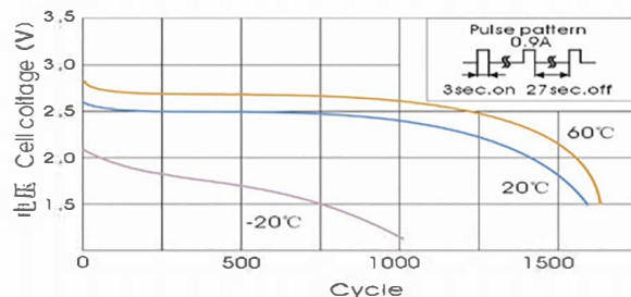
load-Capacity Characteristics
